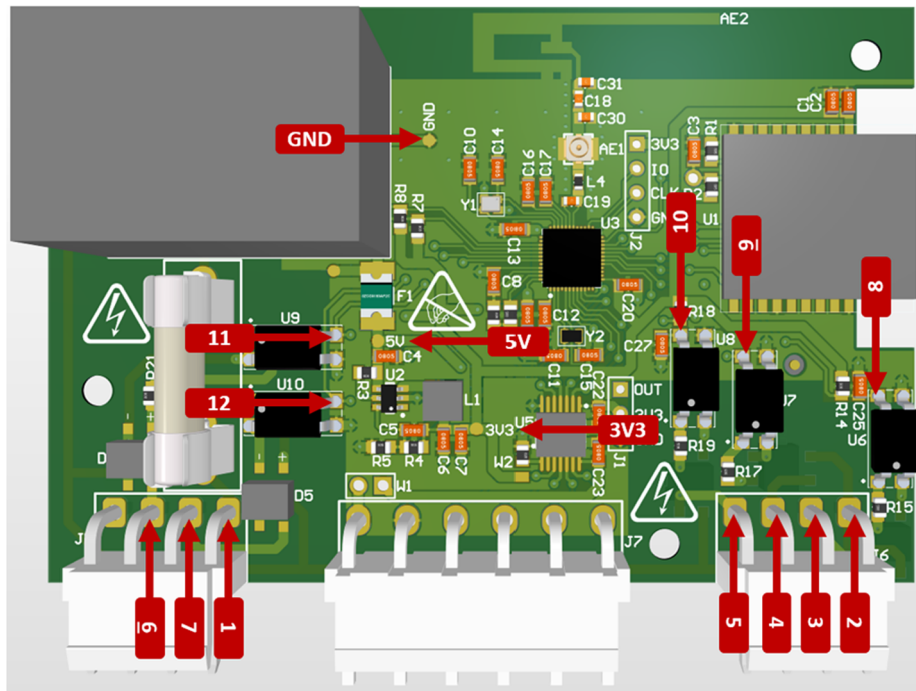
Fig. 13. Points where the IoT-enabled board should be tested.
