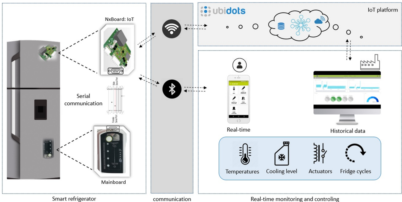
Fig. 3. End-to-end IoT-enabled smart home appliance system.
