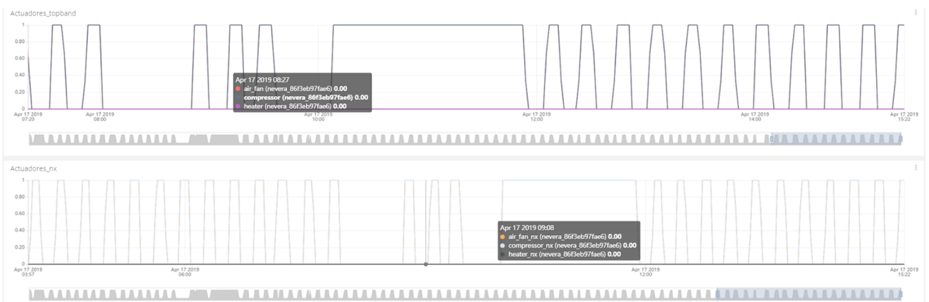
Fig. 11. Comparison between the behaviours of the compressor, defrost heater, and air fan.
