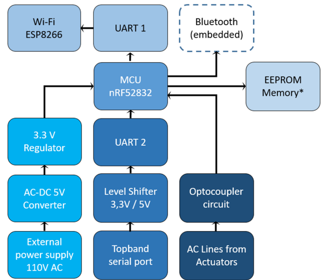
Fig. 6. Hardware architecture for IoT enabled smart home appliance.
