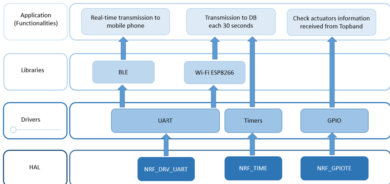
Fig. 7. Firmware architecture for IoT enabled smart home appliance.
