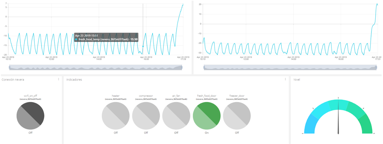
Fig. 10. Fresh food and freezer temperatures with state of actuators including compressor, air fan, heater, fresh food and freezer doors.
