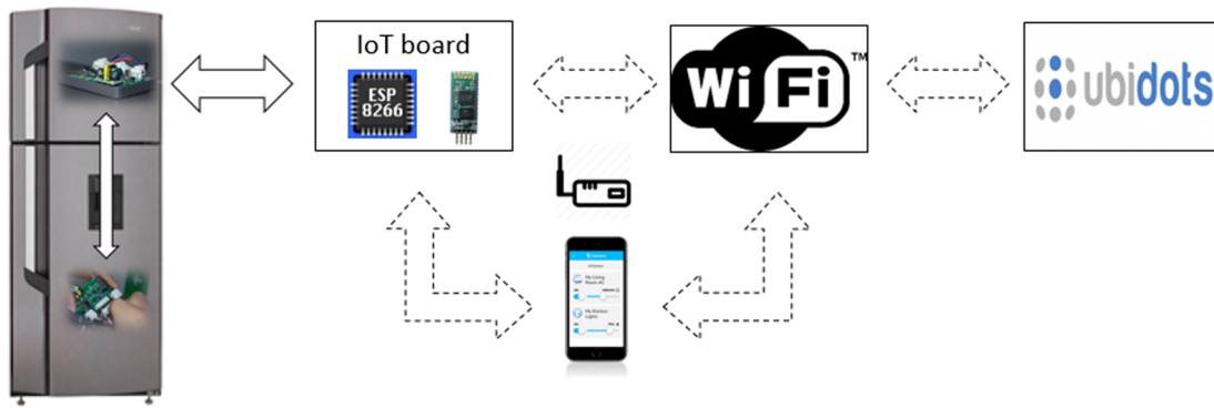
Fig. 5. Wireless network connection and IoT platform enabled smart refrigerator.
